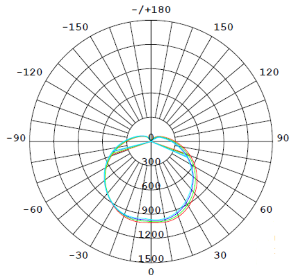
Luminous Intensity Distribution Graph
