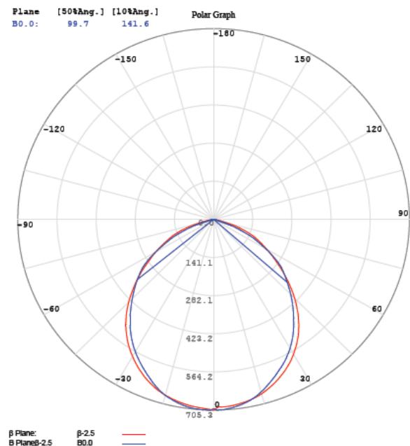
Luminous Intensity Distribution Graph
