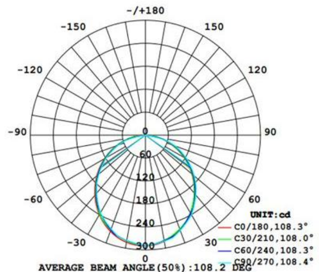
Luminous Intensity Distribution Graph
