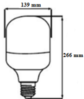
Dimensional Drawing
