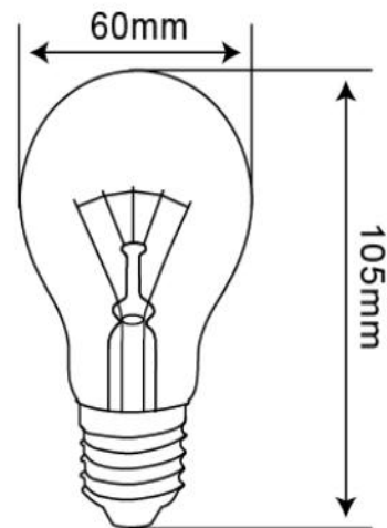
Dimensional Drawing
