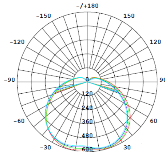
Luminous Intensity Distribution Graph
