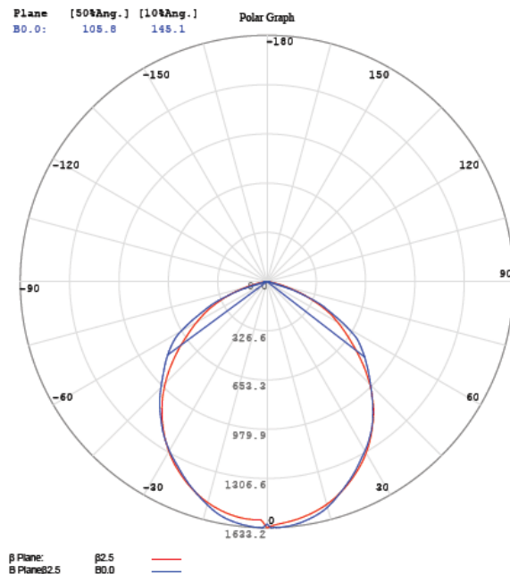
Luminous Intensity Distribution Graph
