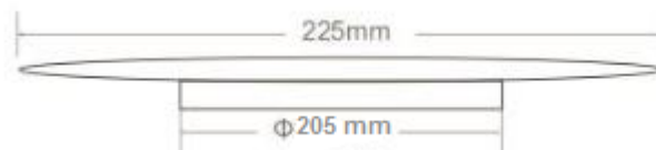
Dimensional Drawing
