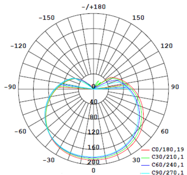
Luminous Intensity Distribution Graph
