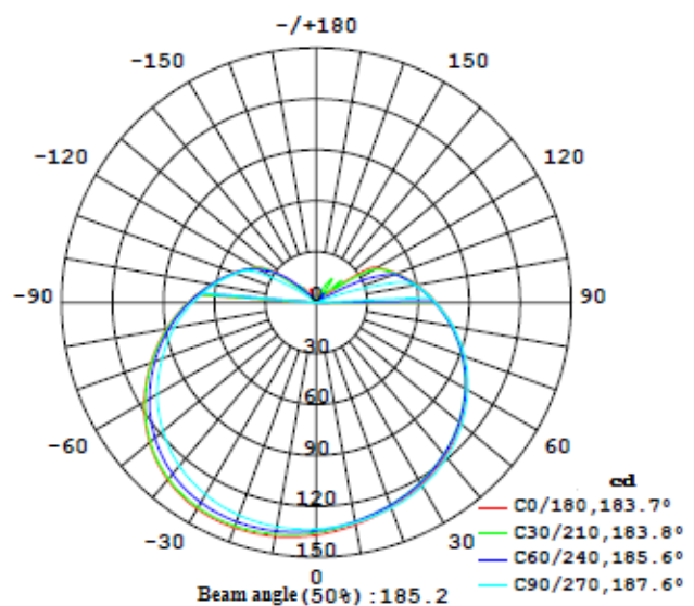
Luminous Intensity Distribution Graph
