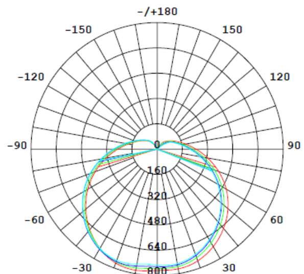
Luminous Intensity Distribution Graph
